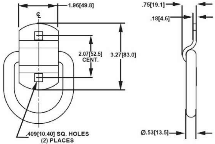
TREIL866ZN Steel, Zinc Plated
